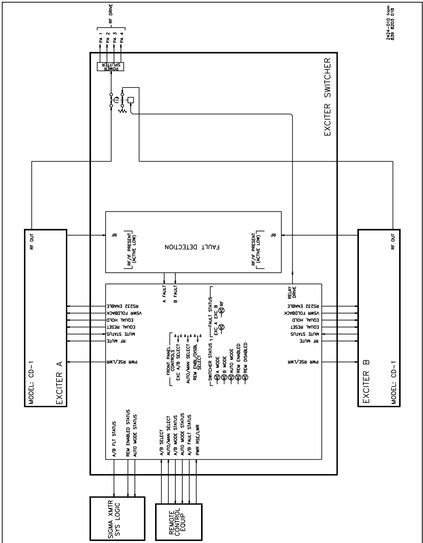
Figure 1-1. Block Diagram, Exciter Switcher
