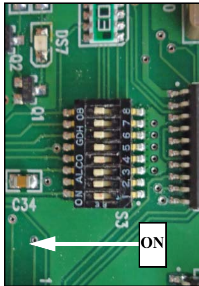
Figure 2-3 S3 Shown With All Switches Closed ("Zero"/ ON)
