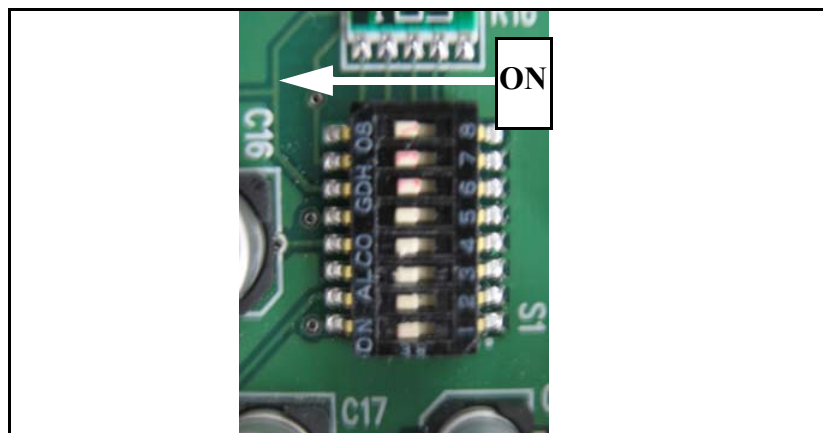
Figure 2-2 S1 Shown With All Switches Closed ("Zero"/ON)
