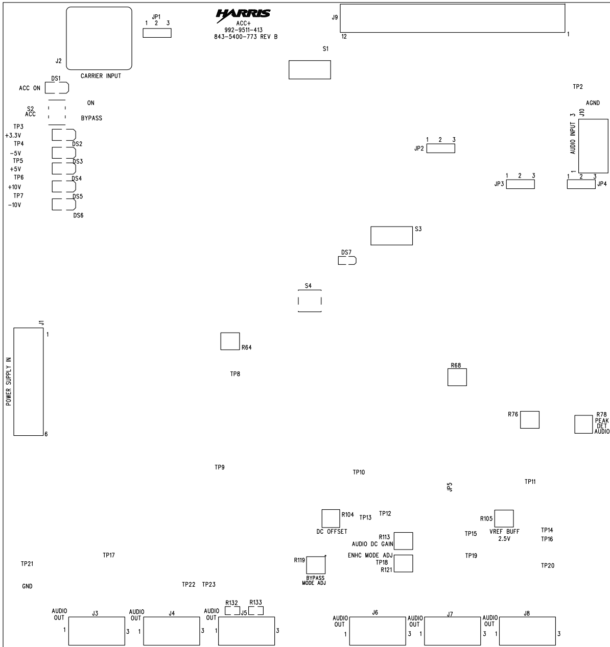
Figure 3-1 Component Locator
