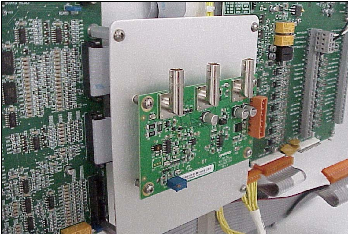
Figure 2-1 Typical AM DAB Switch with PLL Board Location
