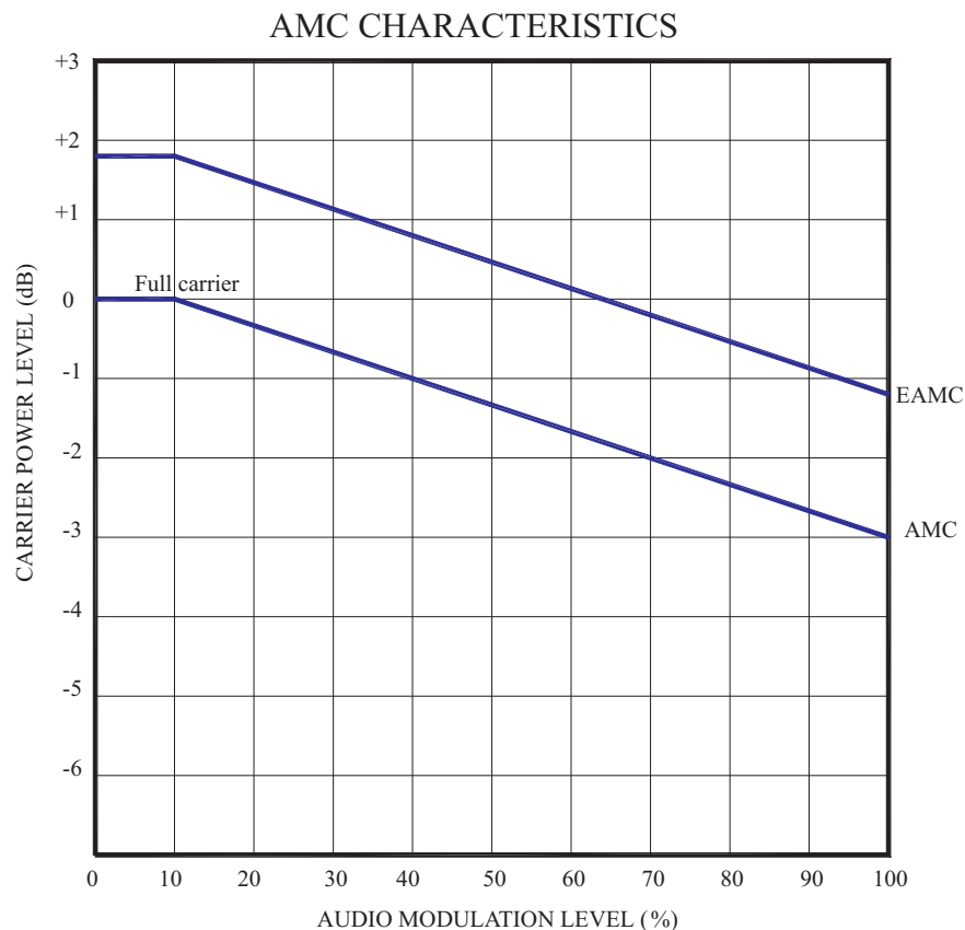
Figure 1-1 AMC+ Characteristics Curve Graph
