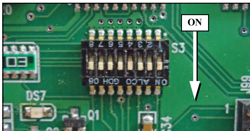
Figure 2-3 S3 Shown With All Switches Closed (zero/ON)
